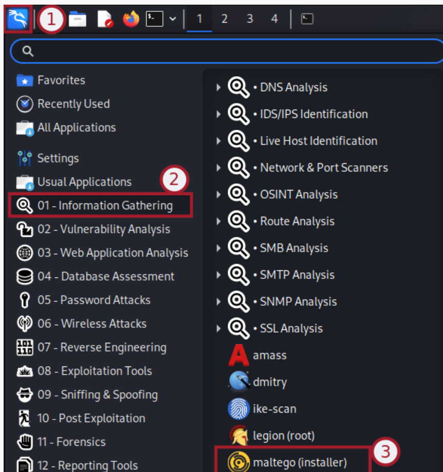
Image 1: Starting maltego (installer)
